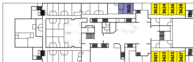
3 – Pont Principal (Main Deck)
